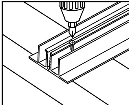
2 Install base
